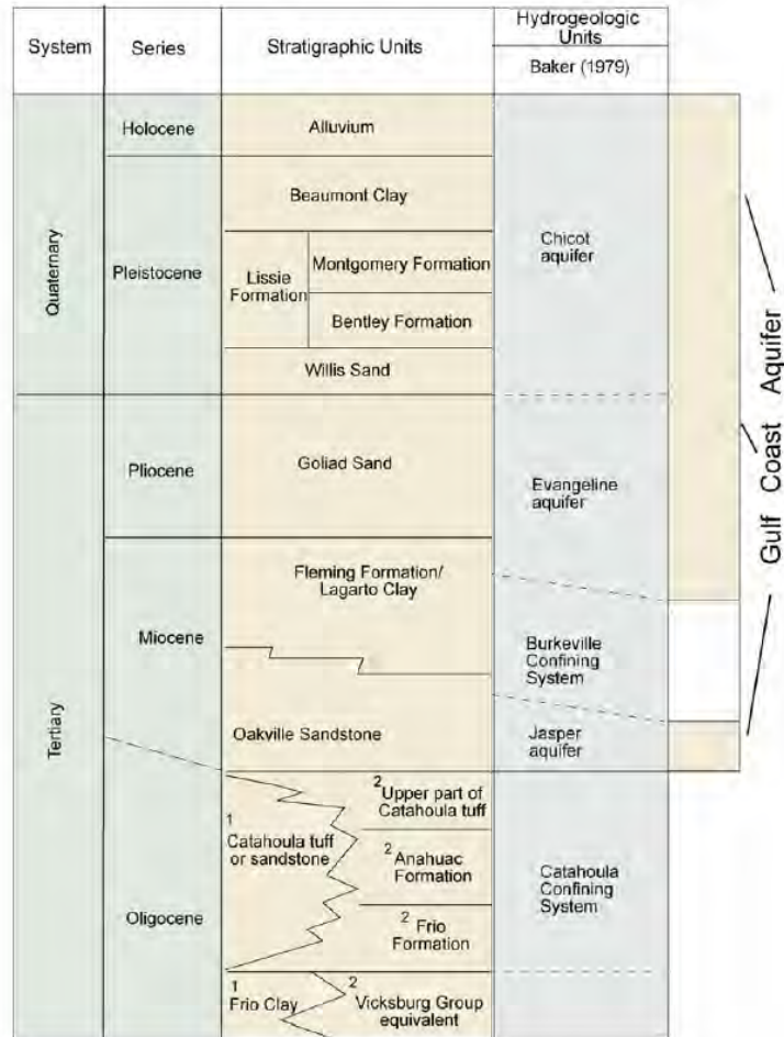
Figure 40. Stratigraphy and hydrostratigraphy of the Gulf Coast aquifers
