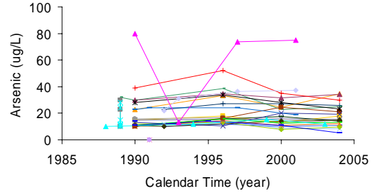
Figure 7. Time series for arsenic analyses (a) south of southern High Plains; (b) southwestern Gulf Coast (both from TWDB database)
